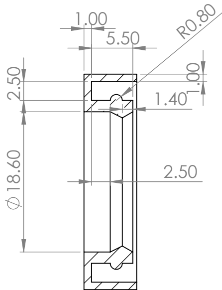
SECTION B-B
